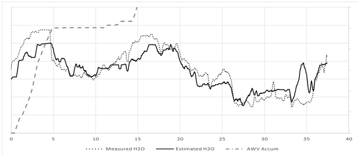
Figure 12. Estimated vs. measured water vapor after a gunning event.
